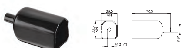
Insulation Boot
