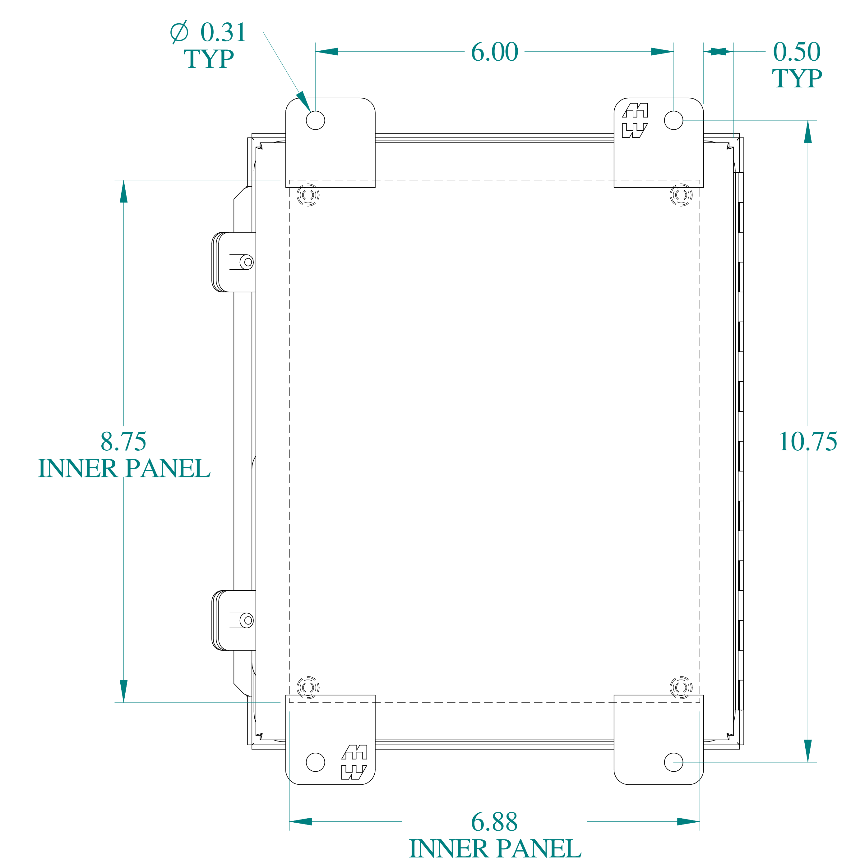
BACK VIEW
