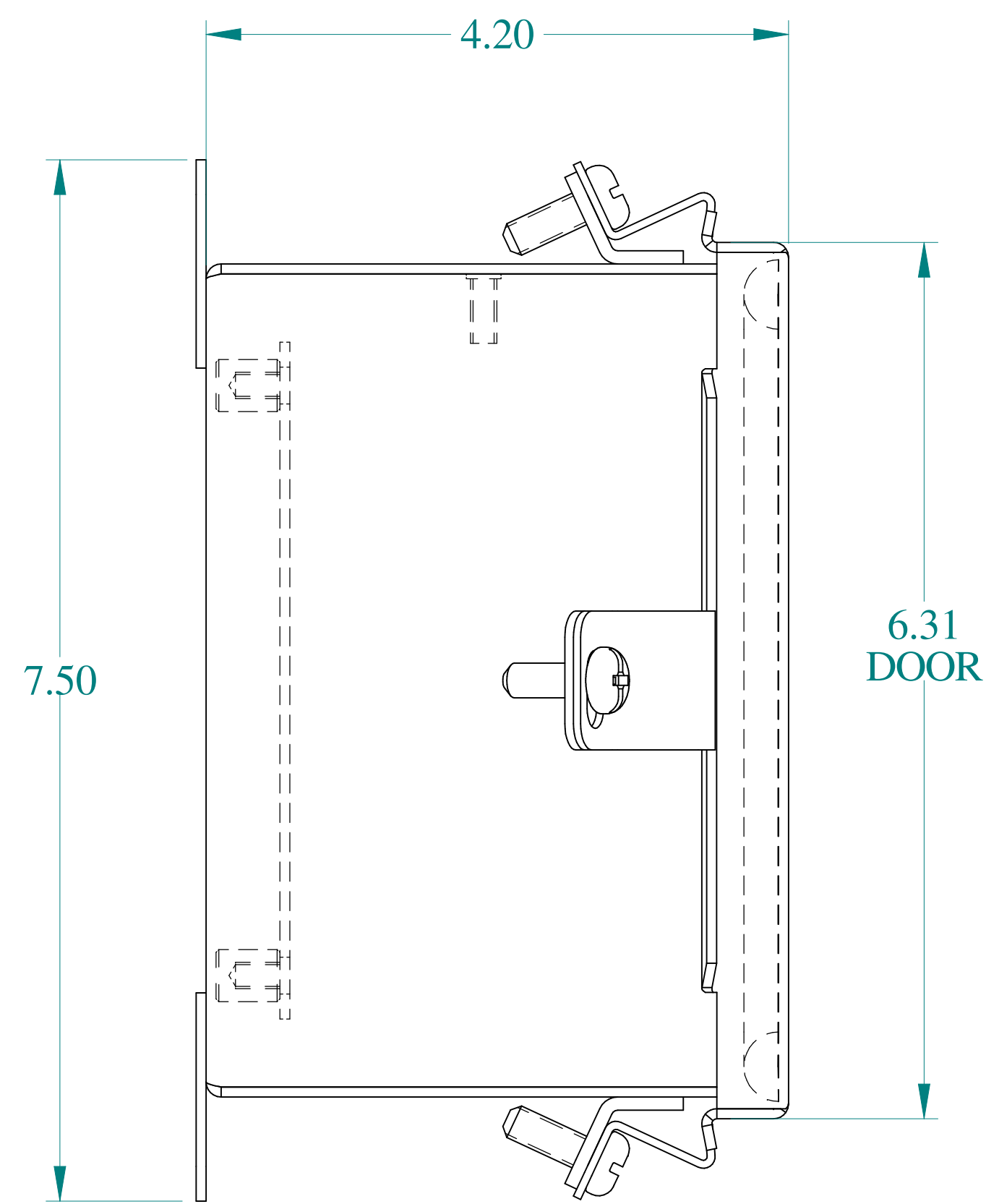
SIDE VIEW
