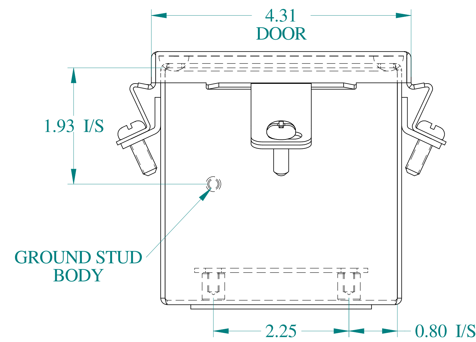
BOTTOM VIEW
