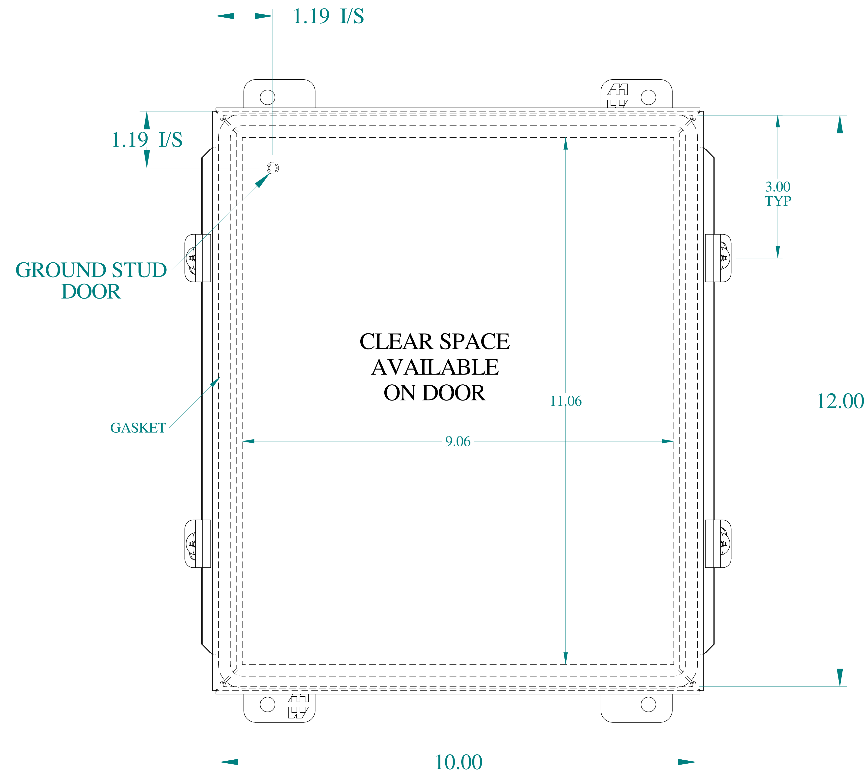
FRONT VIEW
