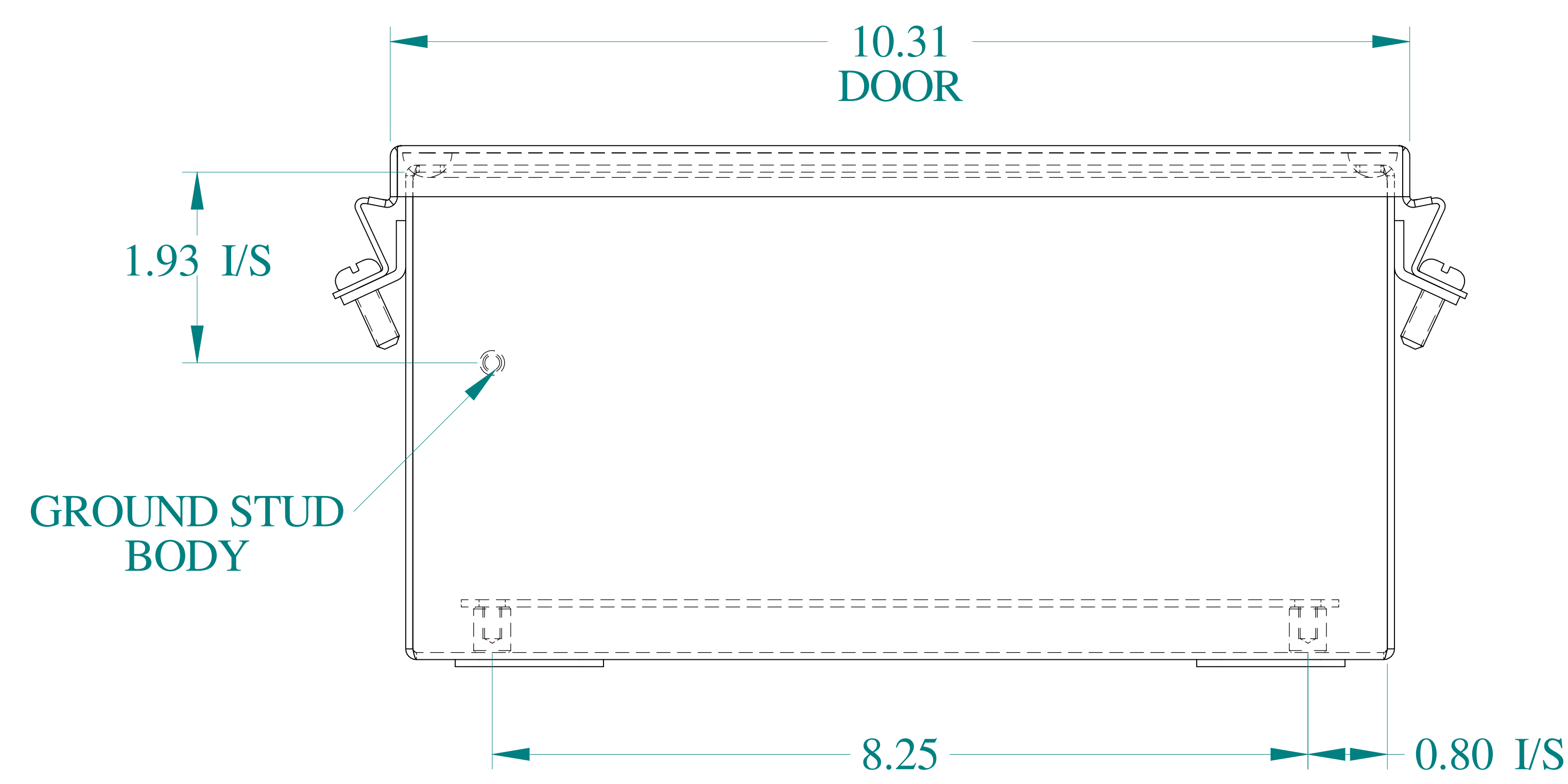
BOTTOM VIEW
