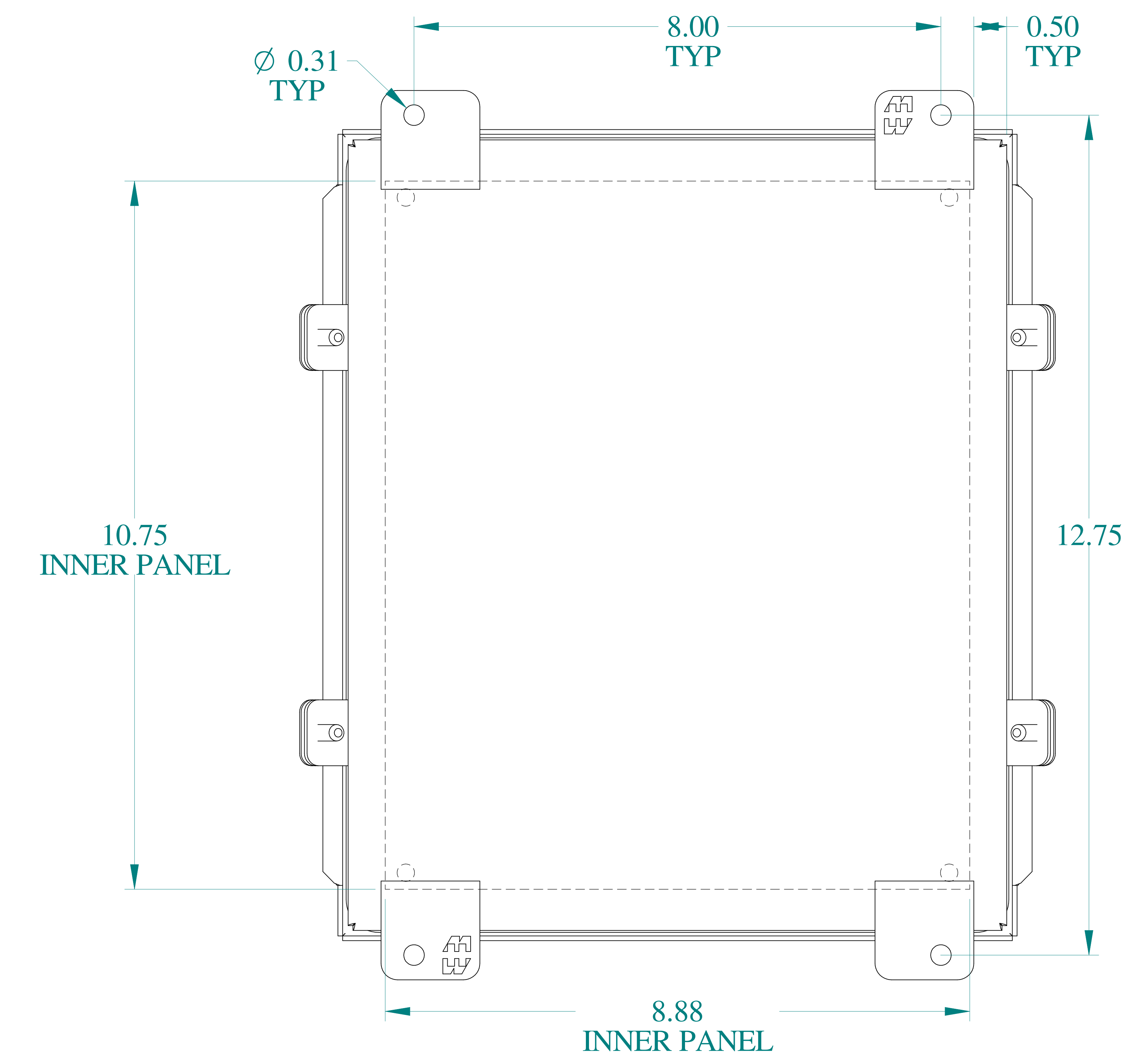
BACK VIEW
