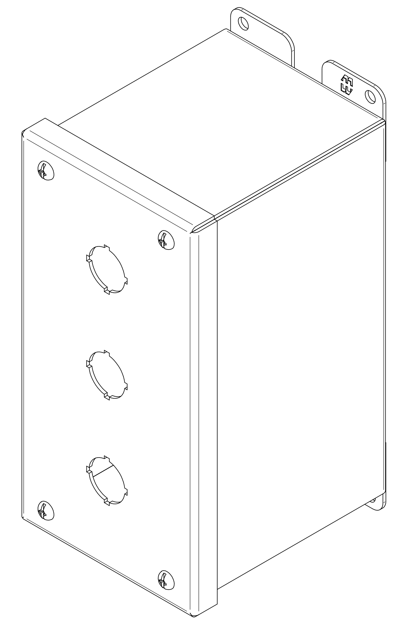
ISOMETRIC VIEWS
