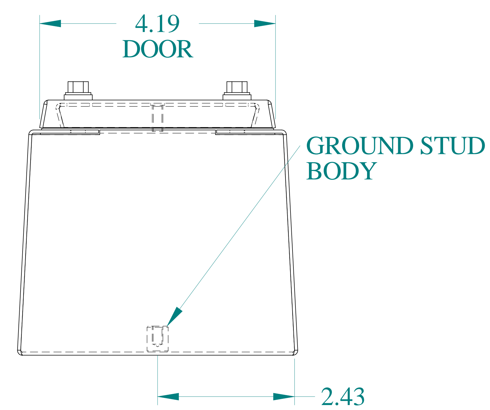
BOTTOM VIEW
