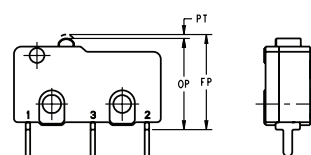
Terminal Type 20
