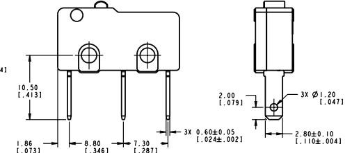
Terminal Type 70 - Long Solder
