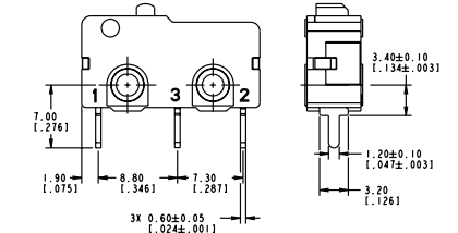
Terminal Type 20 - Straight PCB
