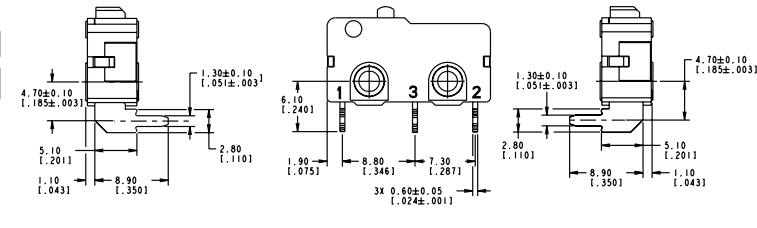
Terminal Type 50 - Right PCB
