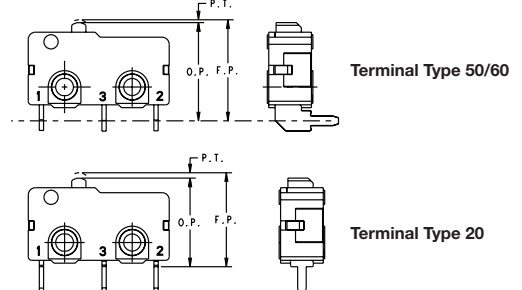
Operate Point References for PCB Terminals
