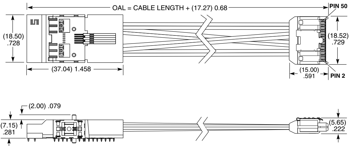
FQSFP-DD-01-X-XX.X-3 SHOWN
