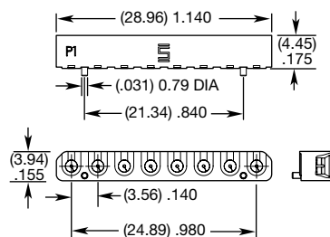
GPPC-PS-1-08-HG-ST-SL SHOWN
