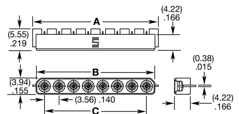
GPPC-PS-1-08-EG-ST-EM-1N SHOWN
