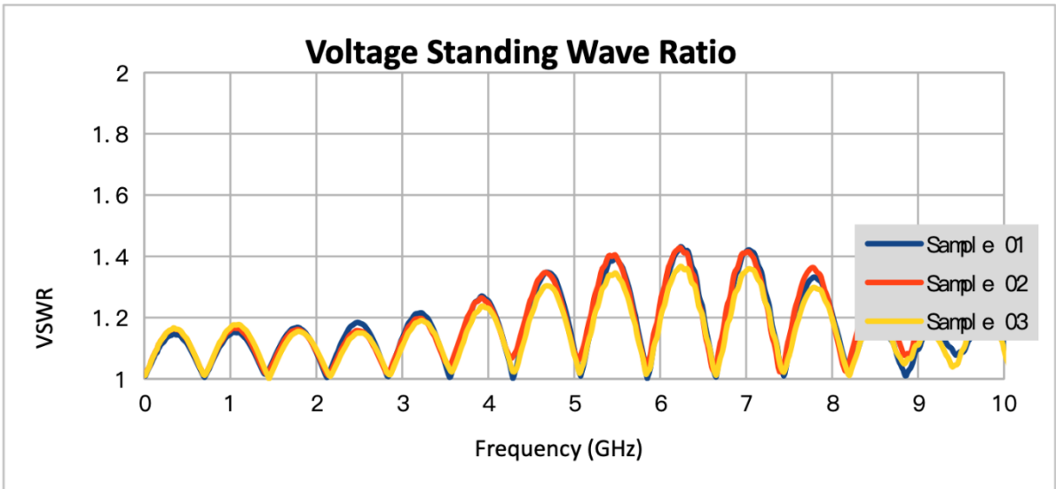
Cable assembly RF058-01SP1-01SP1-0150 (SMA to SMA). See characterization report for more information.
