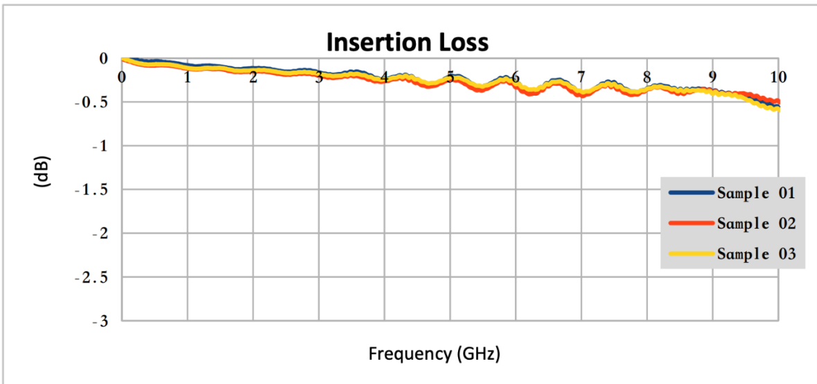
Typical. Results may vary. Includes RF058-01SP1-01SP1-0150 (SMA to SMA) and adaptor effects. See characterization report for more information.
