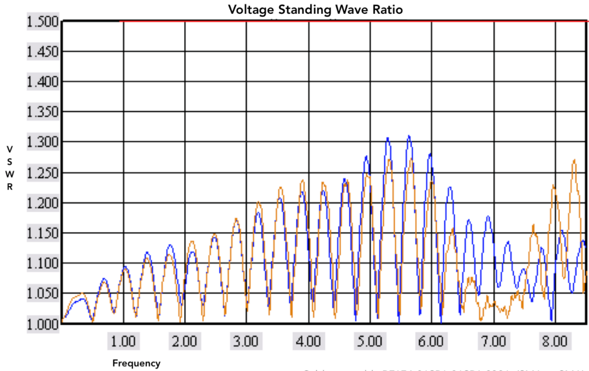
Cable assembly RF174-01SP1-01SP1-0306 (SMA to SMA). See characterization report for more information.
