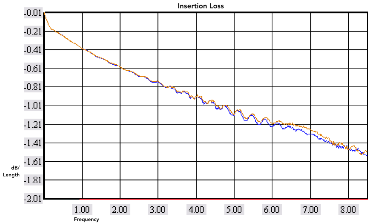
Typical. Results may vary. Includes cable assembly RF174-01SP1-01SP1-0306 (SMA to SMA) and adaptor effects. See characterization report for more information.
