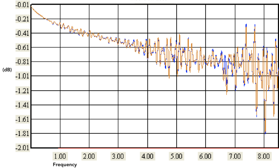
Typical. Results vary. Includes RF179-77RP1-77RP1-0306 (SMB to SMB, Right Angle, 75 Ohm) and adaptor effects. See characterization report for more information.
