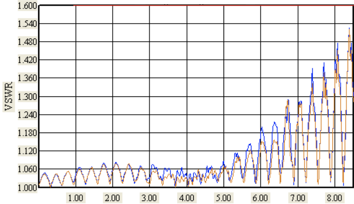
Cable assembly RF179-77RP1-77RP1-0306 (SMB to SMB, Right Angle, 75 Ohm). See characterization report for more information.
