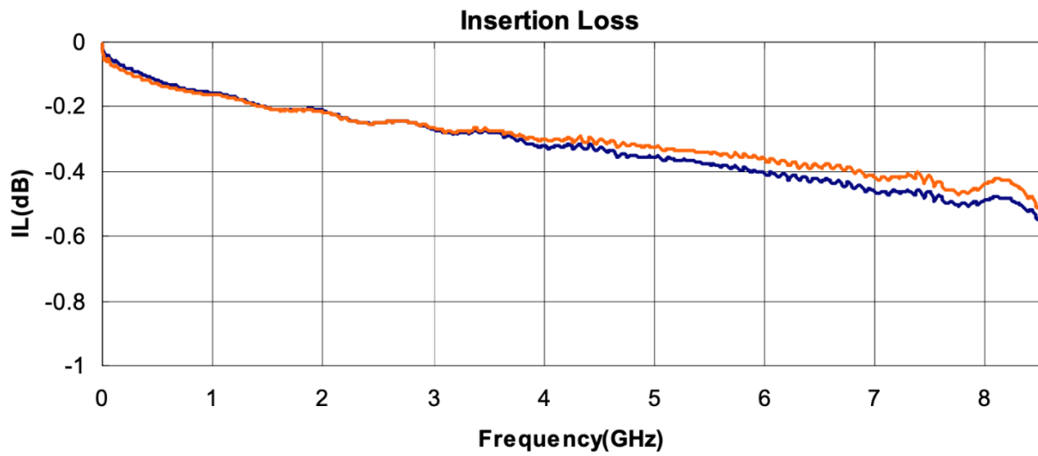
Typical. Results vary. Includes cable assembly RF316-01PN1-01PN1-0150 (SMA to SMA) and adaptor effects. See characterization report for more information.
