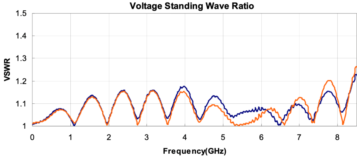
Cable assembly RF316-01PN1-01PN1-0150 (SMA to SMA). See characterization report for more information.
